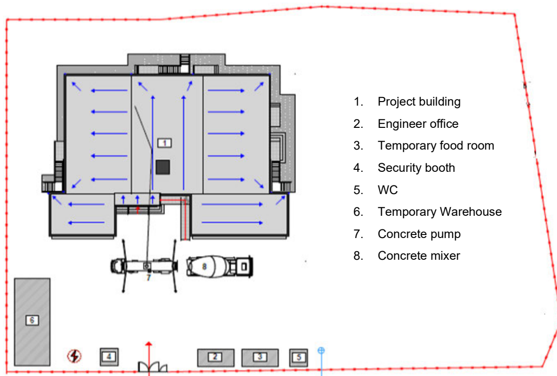
Figure 5 Construction site organization scheme
