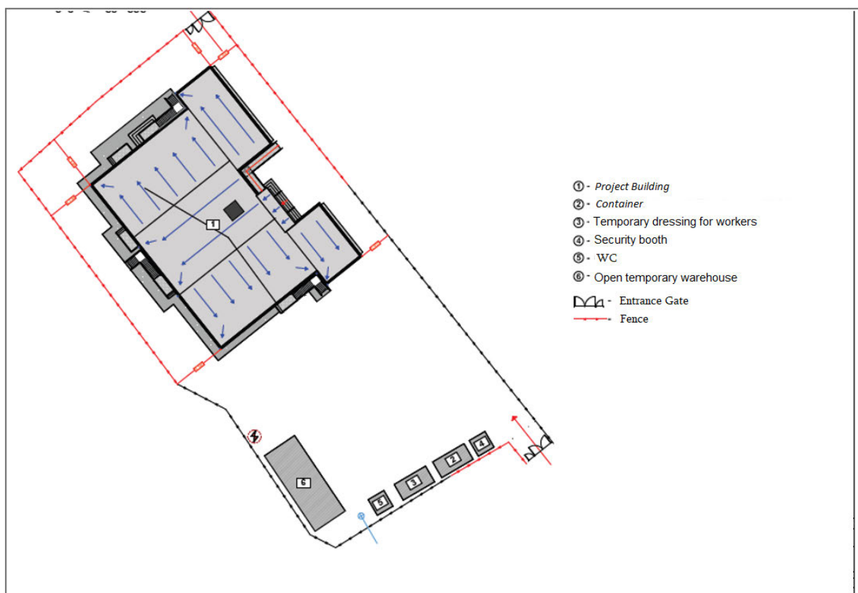
Figure 6. Construction site organization scheme
