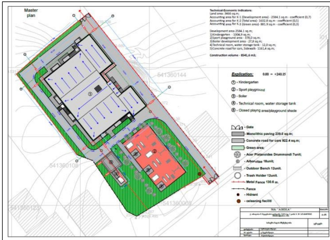
Figure 3 Master Plan
